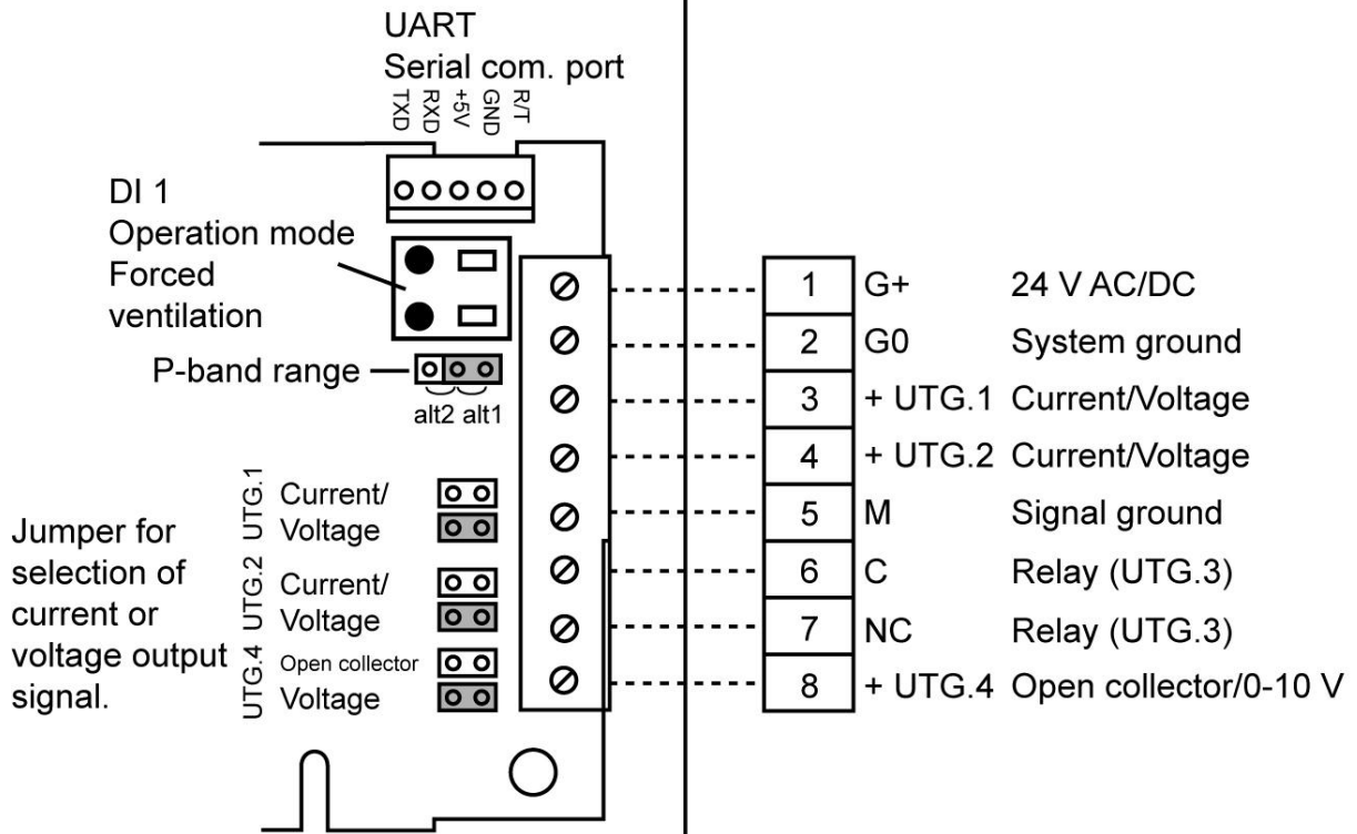
Connection of the UG-M-SENSE III via screw terminal at duct mounting.
